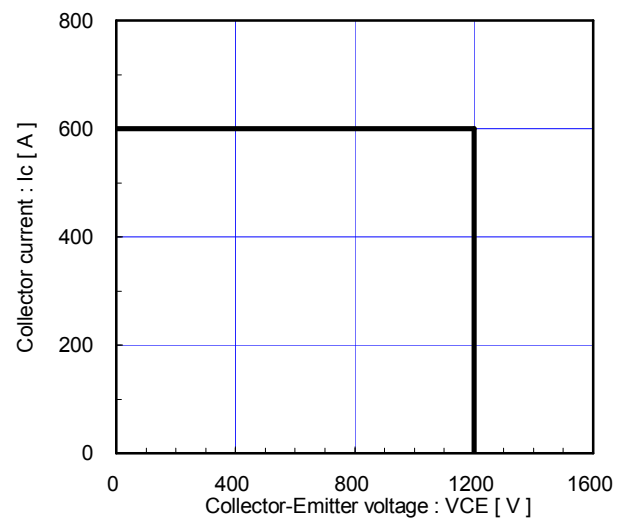
Reverse bias safe operating area (max.) +V_{GE}=15V, -V_{GE} \le 15V, R_G \ge 2.0\Omega, T_j \le 125^\circ C Stray inductance \le 100nH
