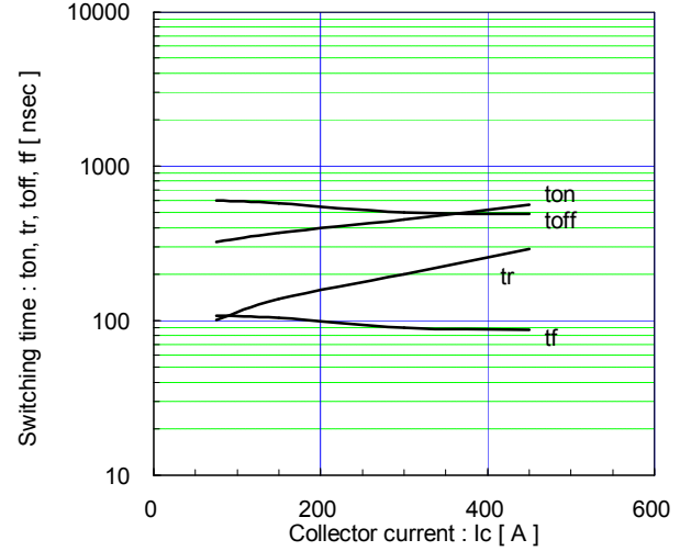
Switching time vs. Collector current (typ.) V_{cc}=600V, V_{GE}=\pm 15V, R_G=2.0\Omega, T_j=125^\circ C
